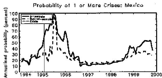
Figure 4: Crisis Probabilities – Total Depreciation (contd.)
